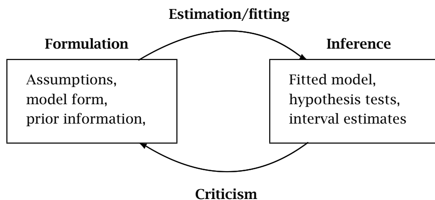
Figure 7.3: Schematic outline of modelling (Cook & Weisberg [4, Fig. 1.2.1])
